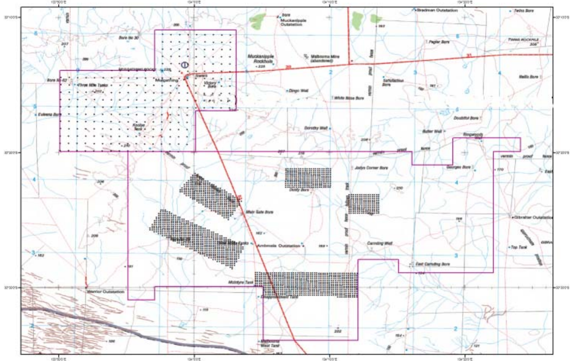
Figure 1. Ambrosia, Mulgathing targeted gravity infill stations
