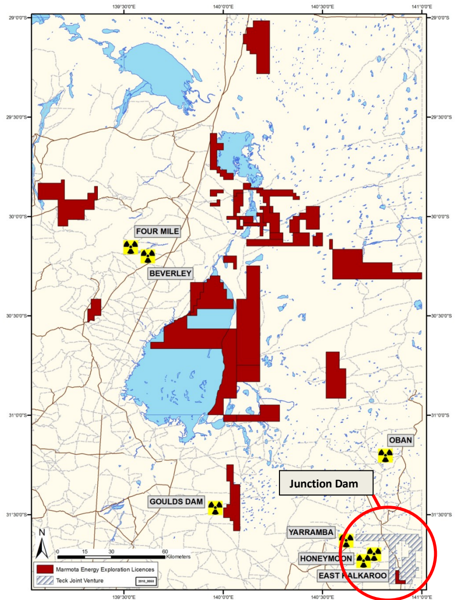
Figure 4: Frome Embayment uranium project locations (red areas) with Junction Dam shown in the grey hash pattern.
