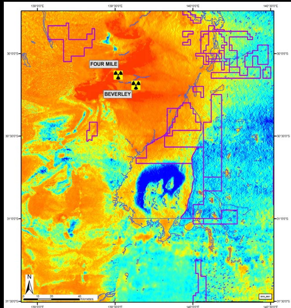
Strong uranium channel radiometric signature (high response: orange – red), Lake Frome region. Marmota tenements outlined in purple.
