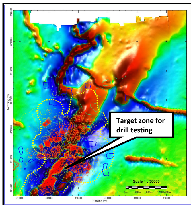
Figure 4: Aurora Tank gold target, gold in calcrete contours over magnetic image. Target area highlighted in yellow dashed line.
