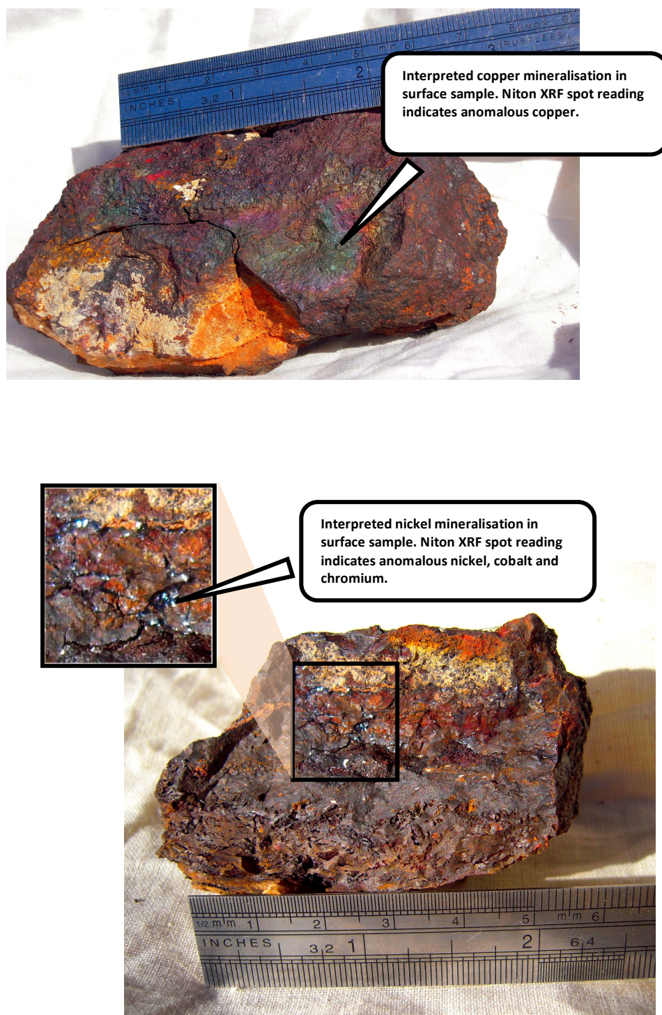
Figure 4: Examples of copper and nickel samples in outcrops from the Durkin area.
