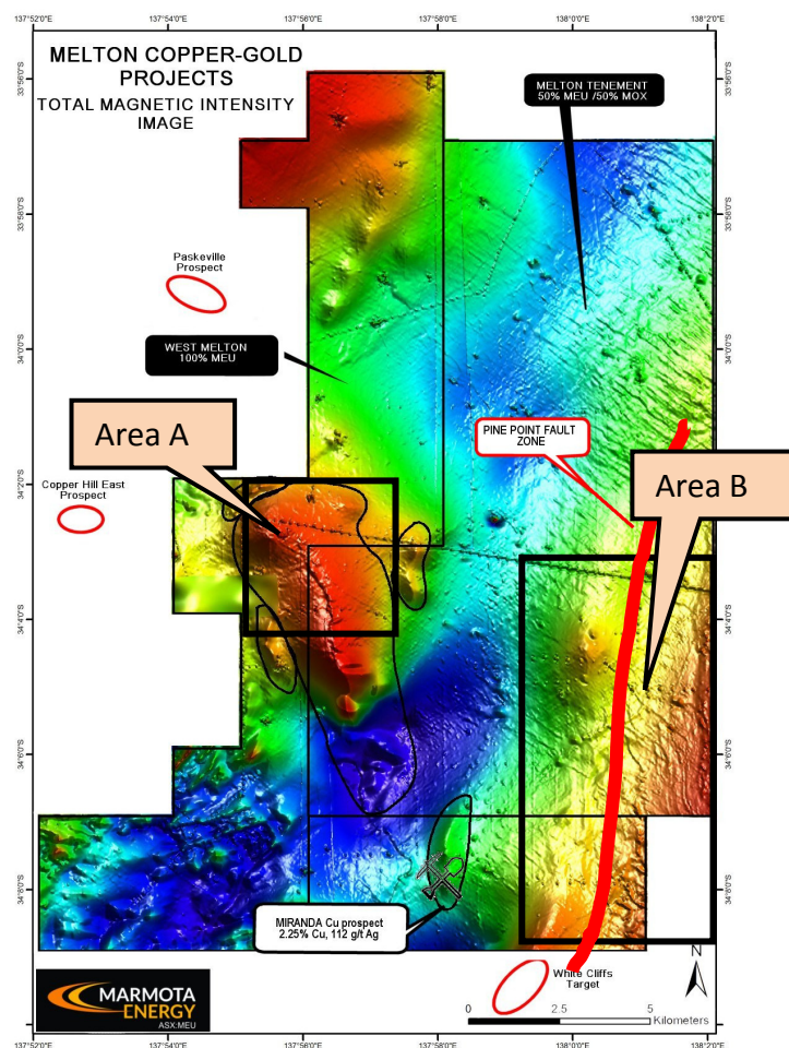
Figure 6b: Melton projects total magnetic intensity image with calcrete sampling areas shown.
