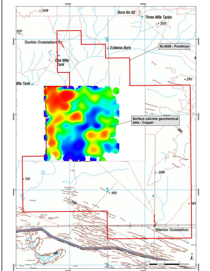
Copper in calcrete anomaly
