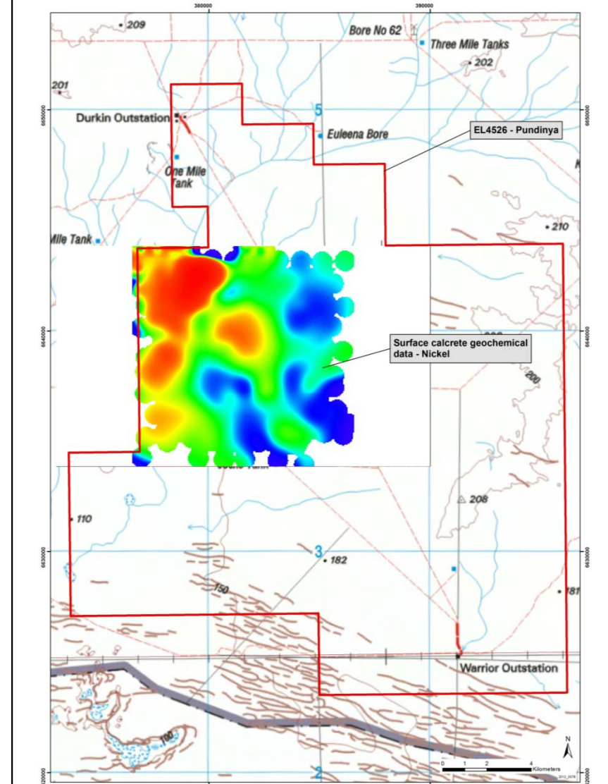
Nickel in calcrete anomaly
