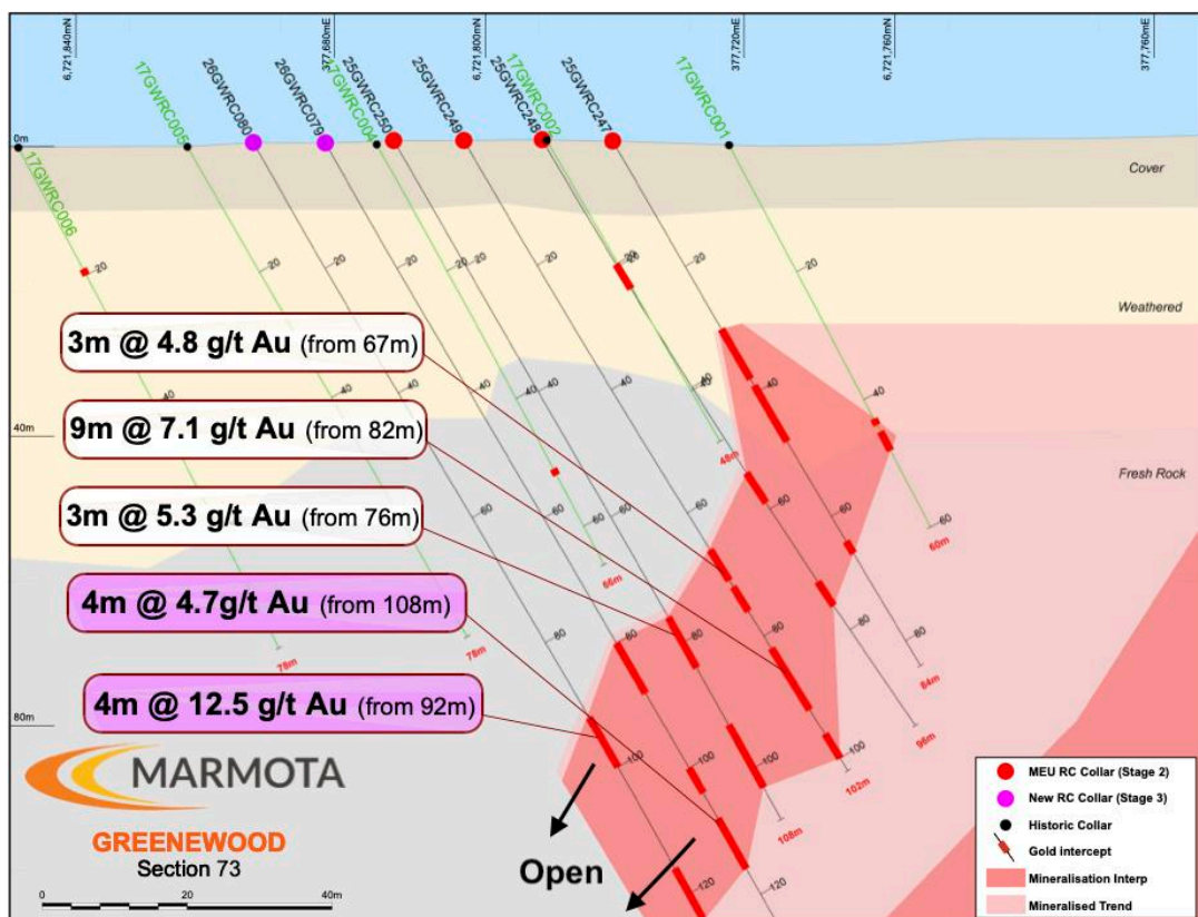
Cross-section 73
