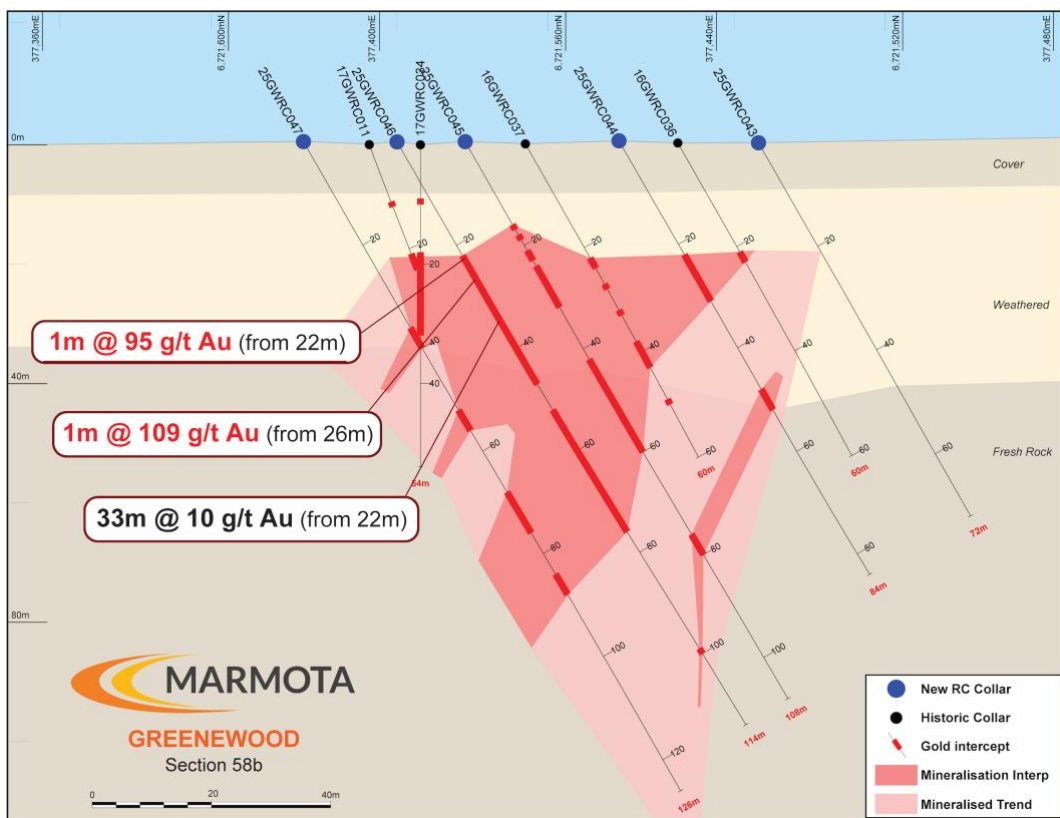
Cross-section 58b
