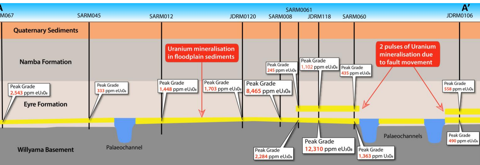
Figure 20: Schematic cross-section with a length of 600 metres across the Saffron Deposit
