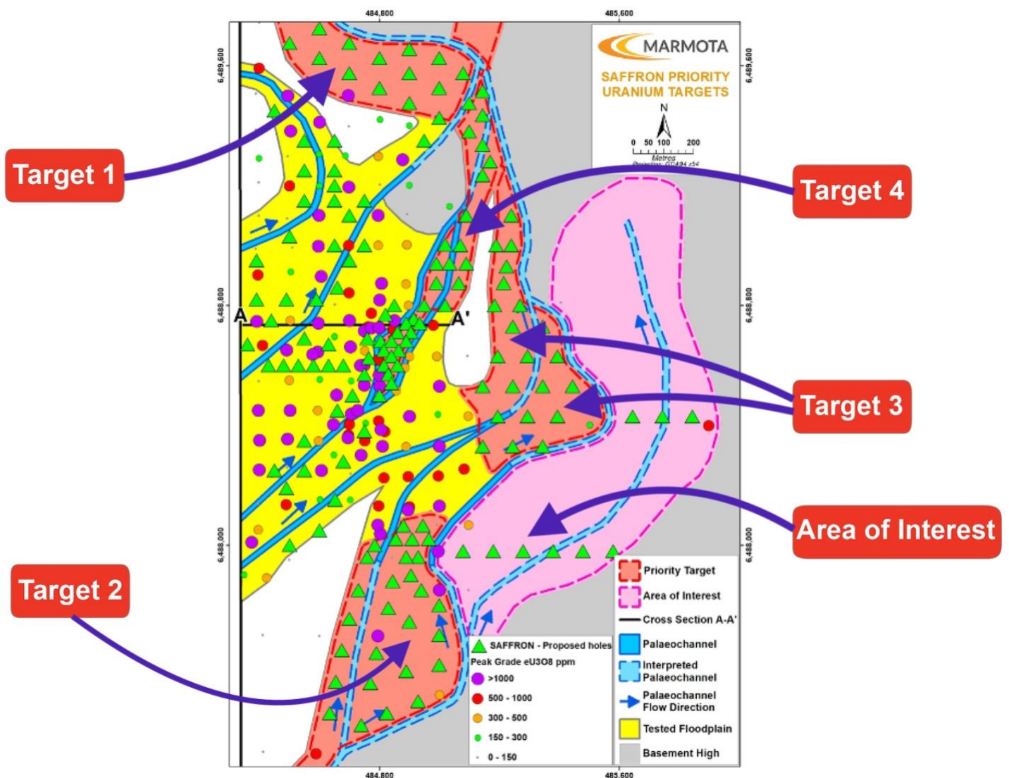
Figure 21: Proposed drill holes ▲ near the Saffron Resource Area including 4 new exploration targets
