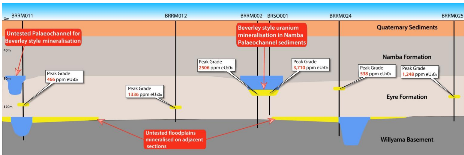
Figure 23: Schematic cross-section across the Bridget Prospect
