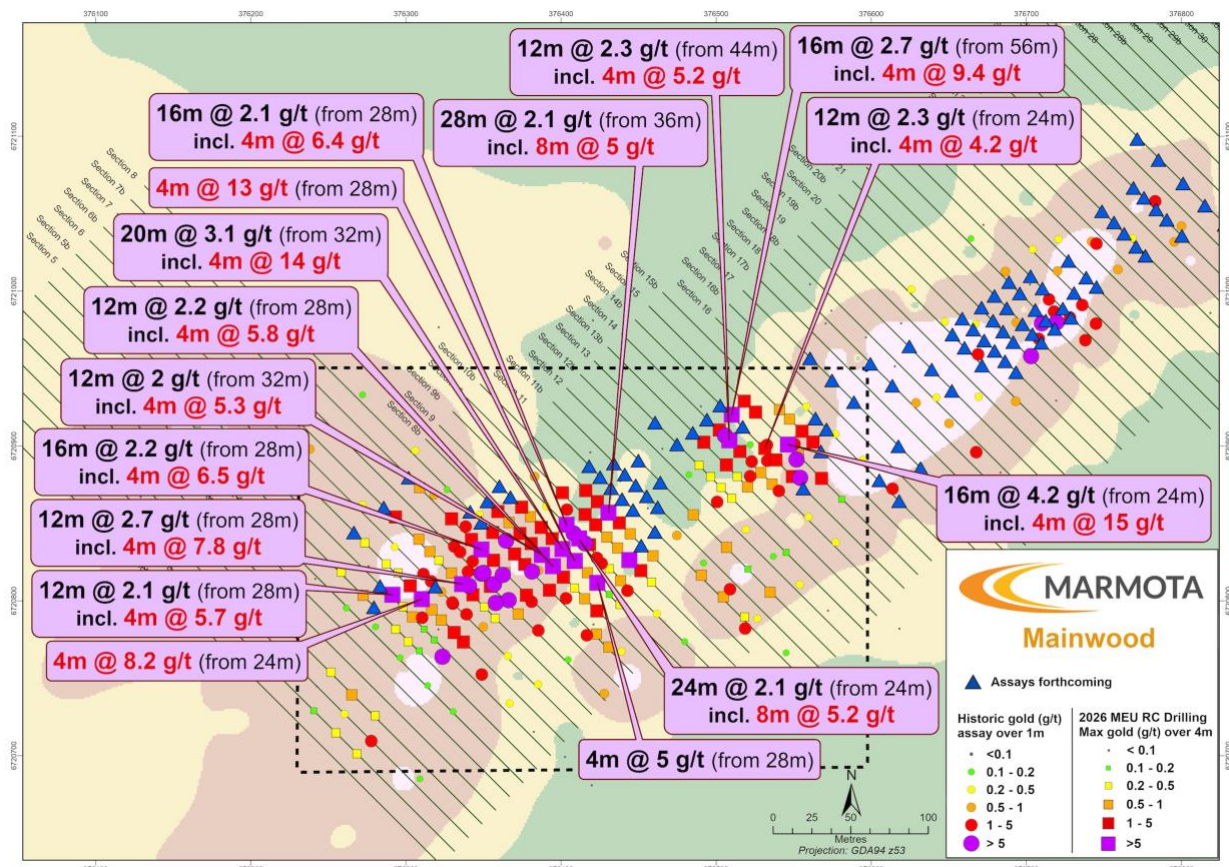
Figure 11: Mainwood Maiden Program – Plan Overview of first results: sections 1 to 15 (Best downhole gold results at collar)
