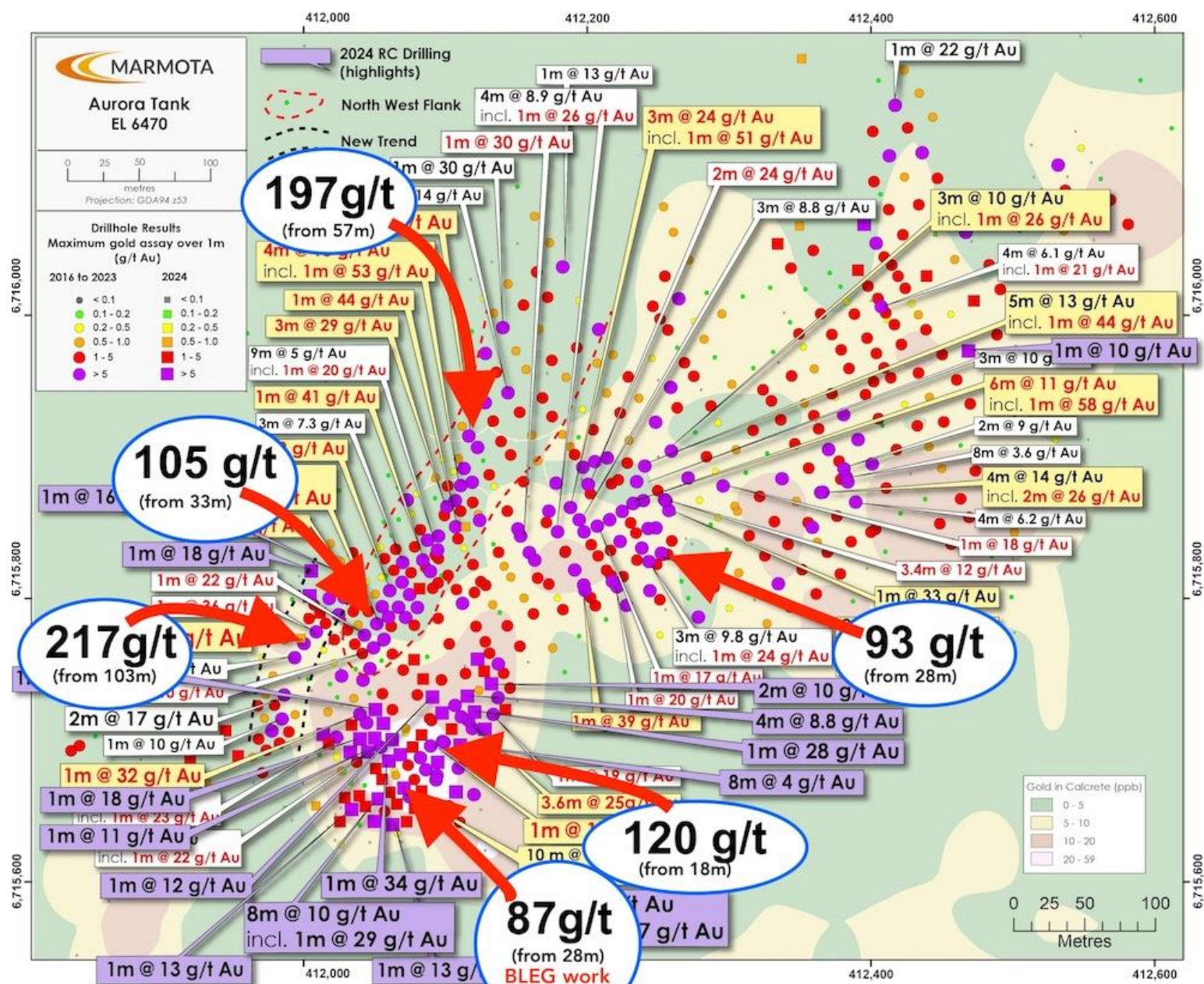
Figure 6: Location and grade of best intersections over 1m (circled) (actual depth from surface) highlighting extensional and infill drilling to the south
