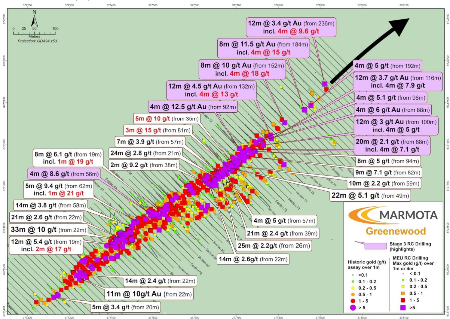
Figure 14: Contiguous high-grade gold strike extends north ... and just keeps going Plan Overview of Greenwood zone, showing northern extensions: sections 48 to 83 (Best downhole gold results at vertical projection)
