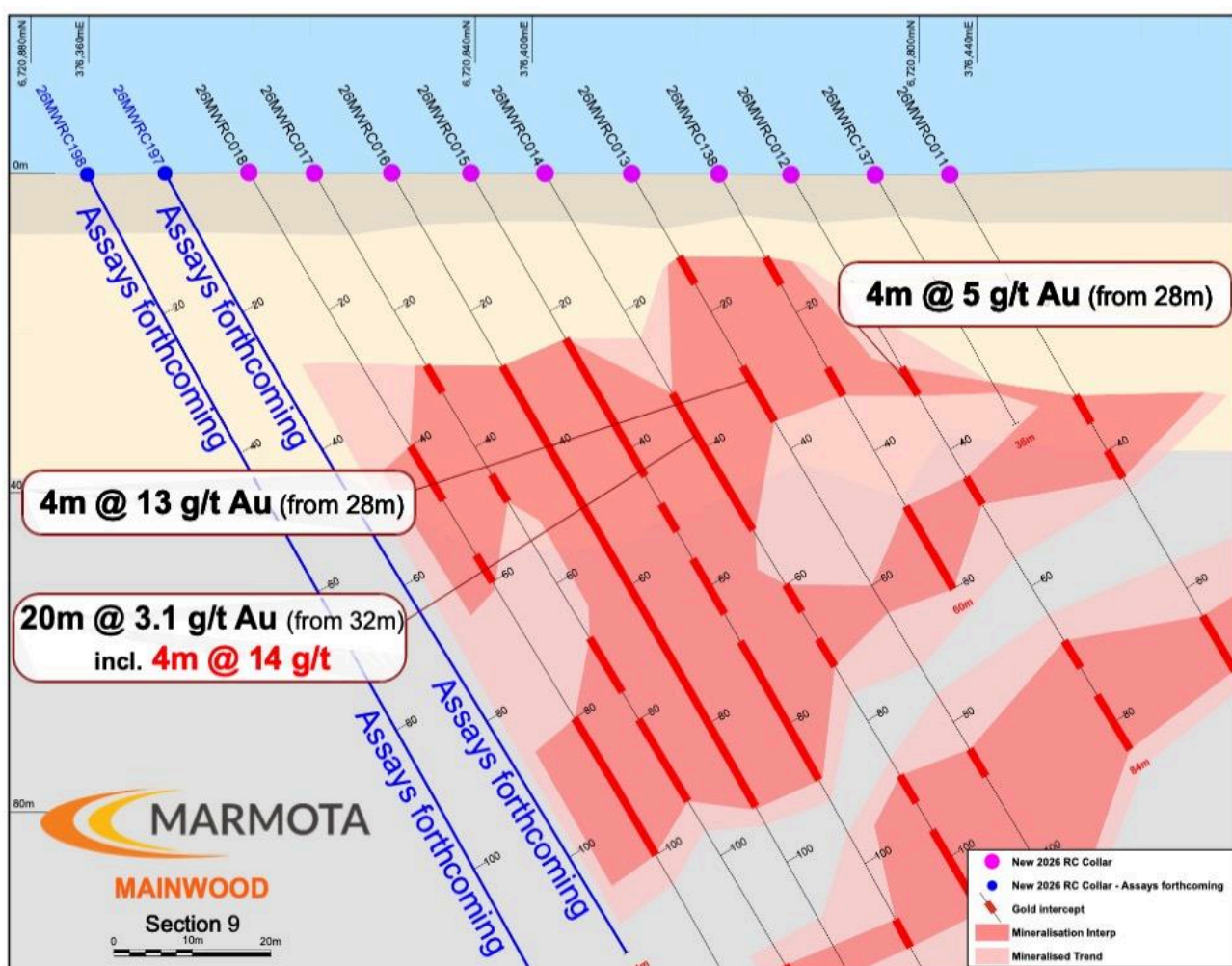
Figure 12: Sectional view through cross-section 9
