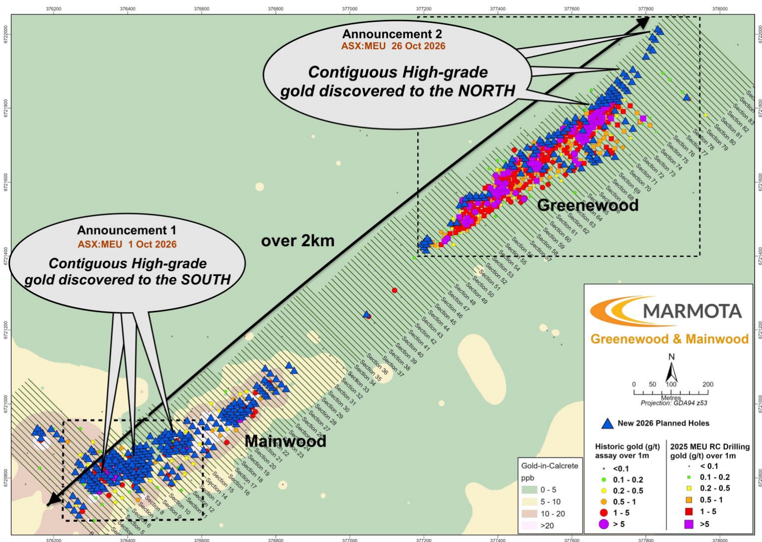
Figure 9: Contiguous high-grade gold discovered to both SOUTH [ ASX:MEU 1 Oct 2026 ] and NORTH [ ASX:MEU 26 Oct 2026 ] 2026 drilling yields massive extension to known high-grade strike
