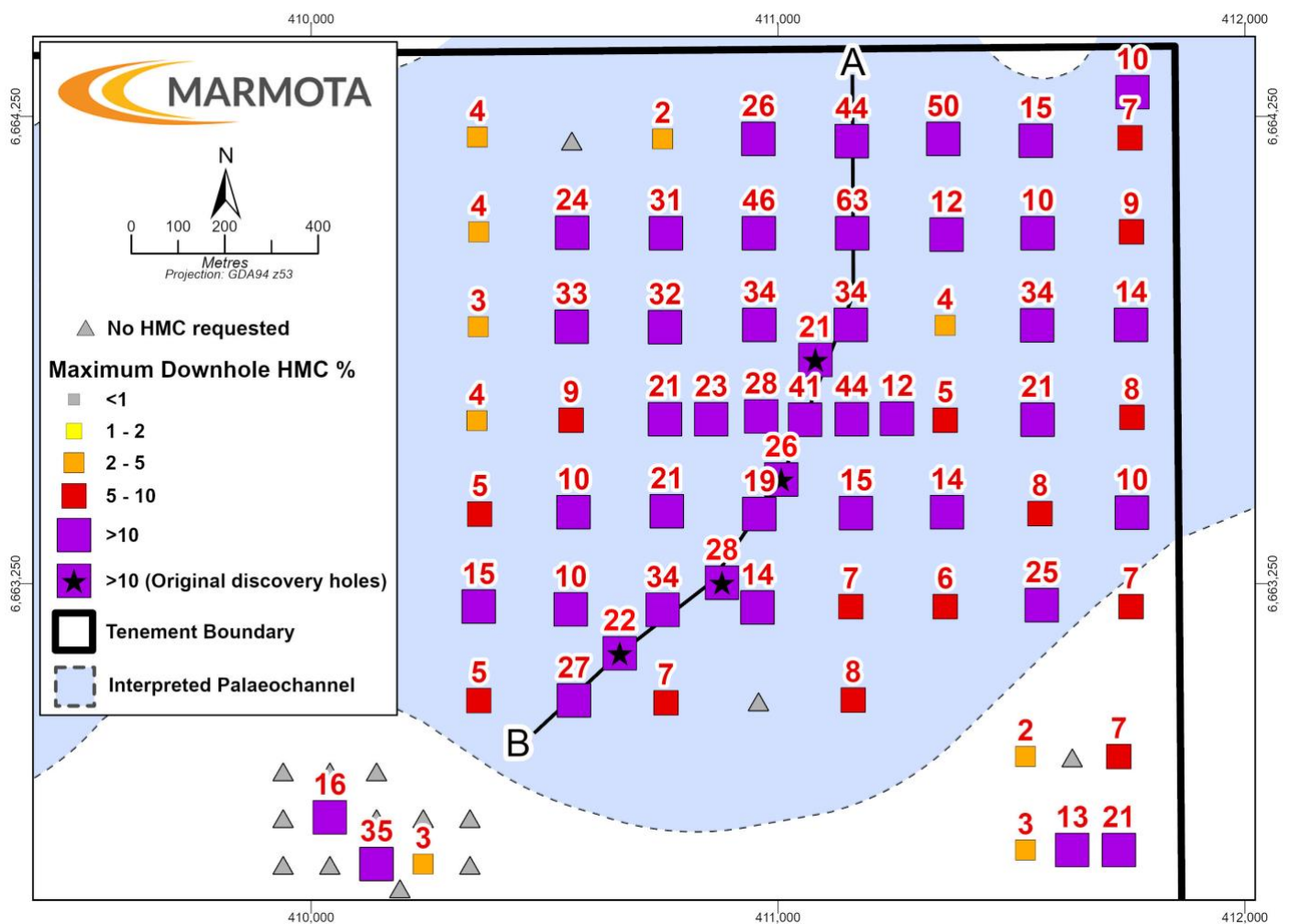
Figure 18: DETAIL VIEW: Ultra-high grade area on MEU Titanium Discovery on EL 6166 (Muckanippie) with interpreted palaeochannel
