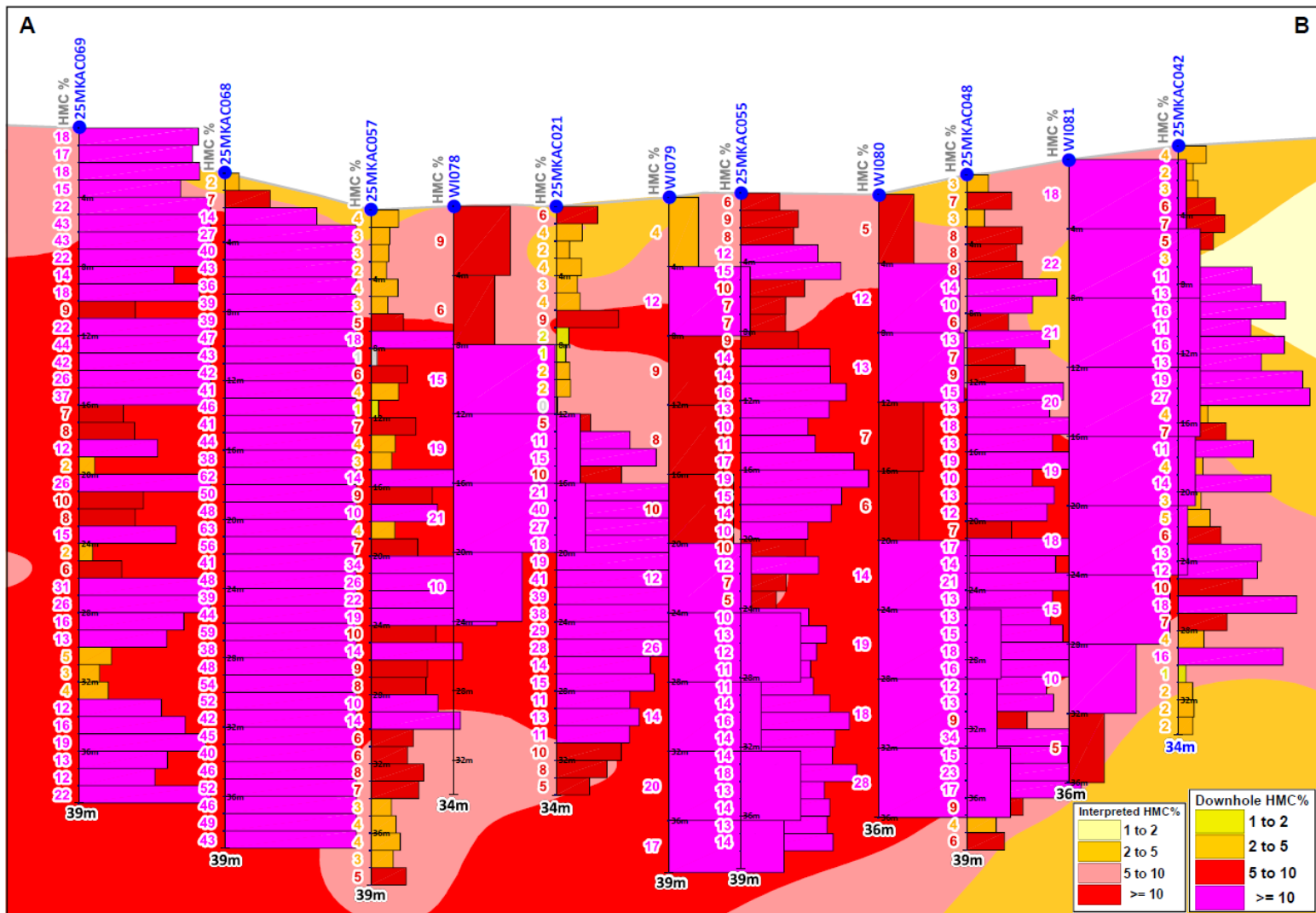
Figure 17: Muckanippie Titanium discovery
