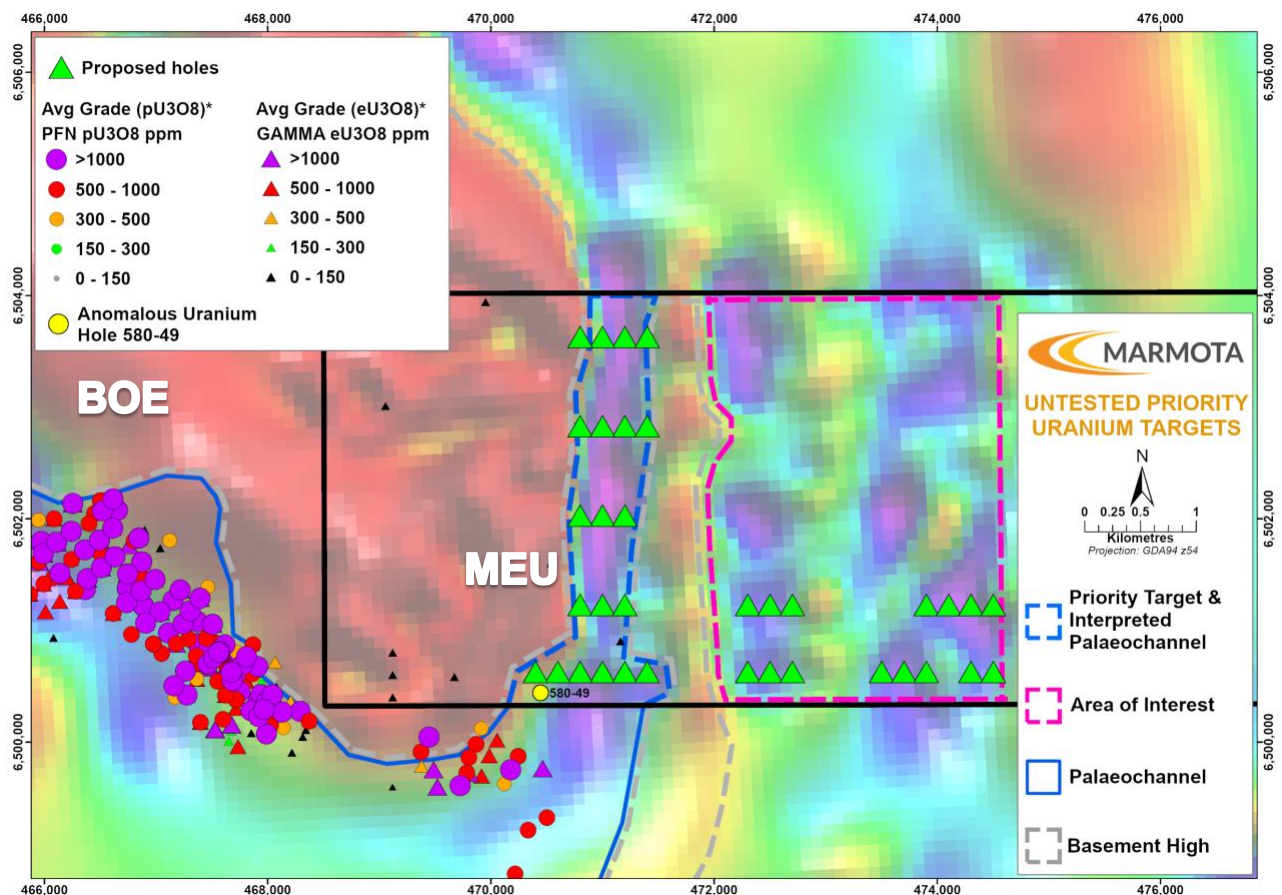
Figure 24: Interpretation of the Jason's region showing priority target
