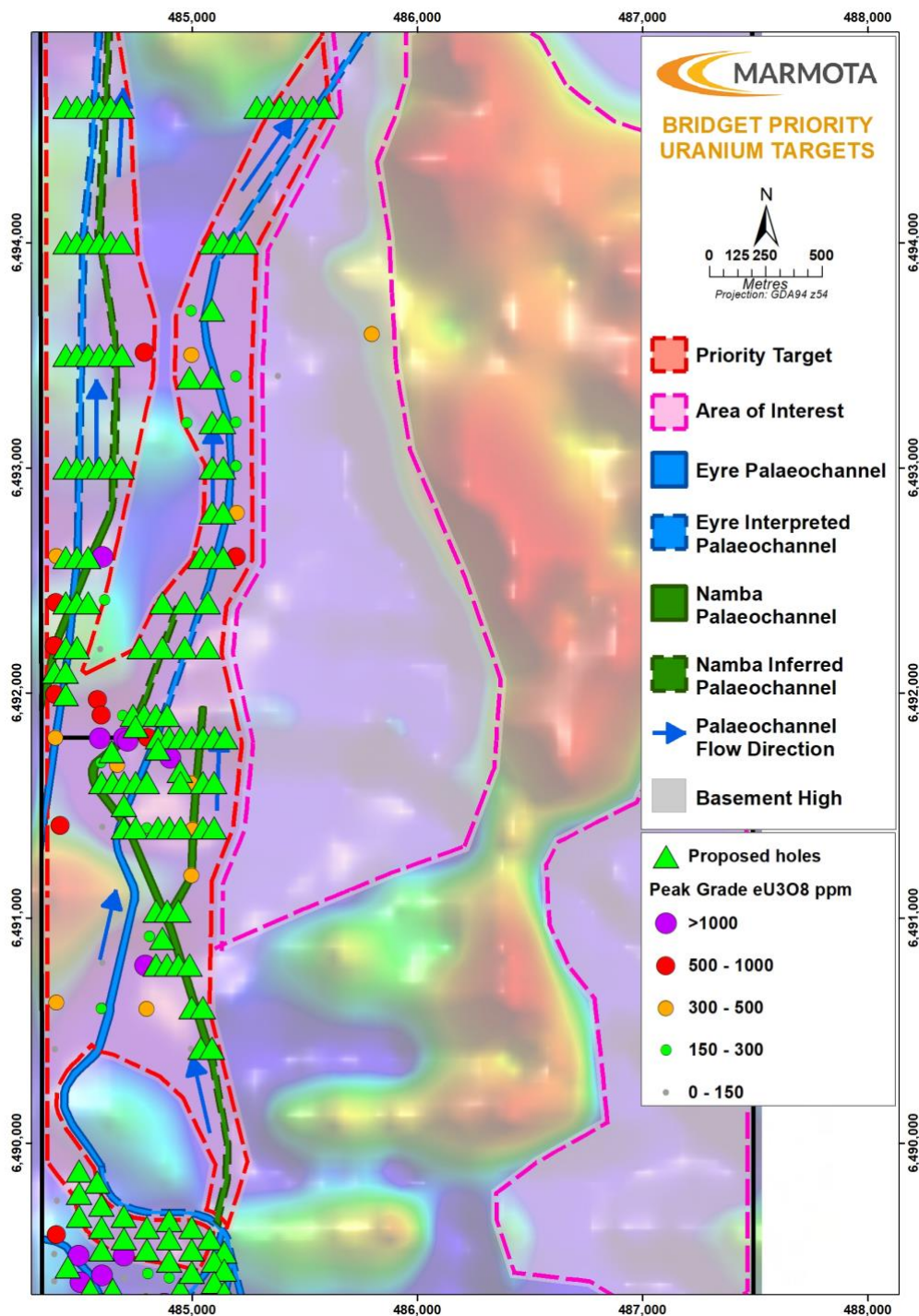
Figure 22: Planned drill holes: Bridget area
